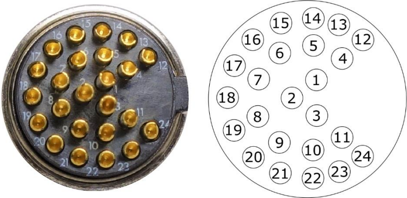
Figure 3: Fischer 24-pin PLUG-connector (SOLDER SIDE)
