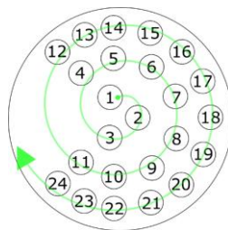
Figure 6: Wire order for soldering Fischer SOCKET connector ( solder side ). Notice that pin order is reversed in PLUG connector.
