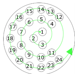
Figure 7: Wire order for soldering Fischer PLUG connector ( solder side ). Notice that pin order is reversed in SOCKET connector.
