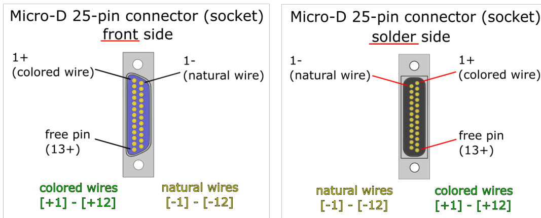
Figure 5: Wire pair order for Micro-D 25-pin SOCKET-connector.
