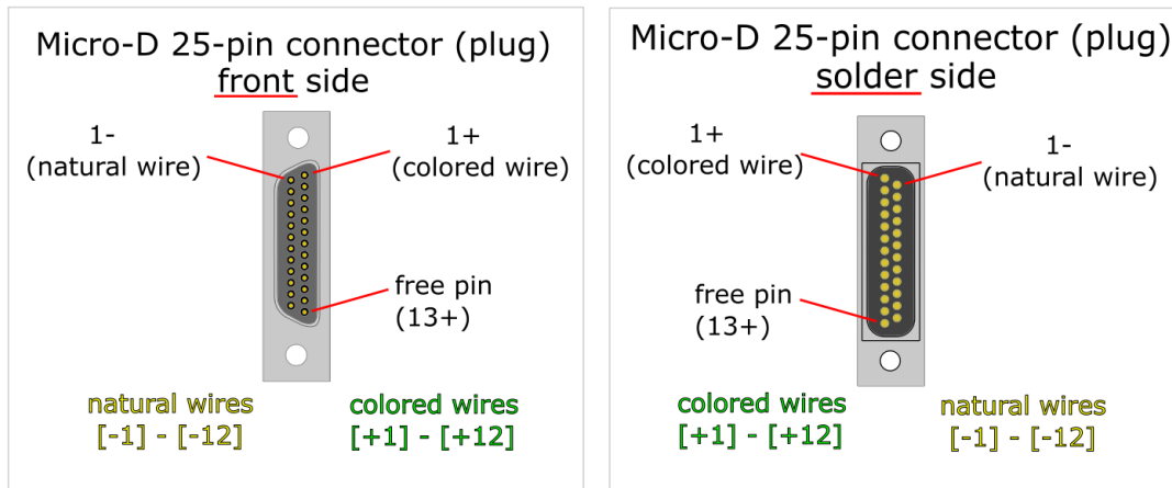
Figure 4: Wire pair order for Micro-D 25-pin PLUG-connector.
